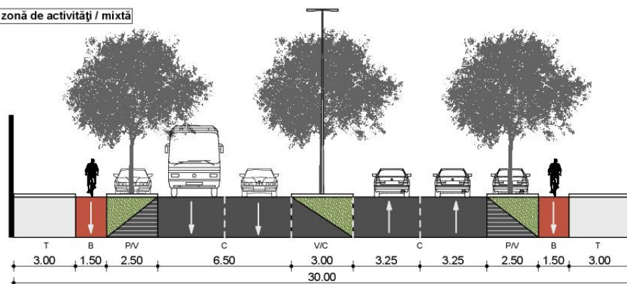
II.D 26m - str. TRAIAN
