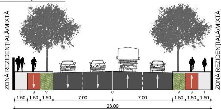
II.K.2 INEL SUDIC, Tronson Mănăstur-Borhanci
